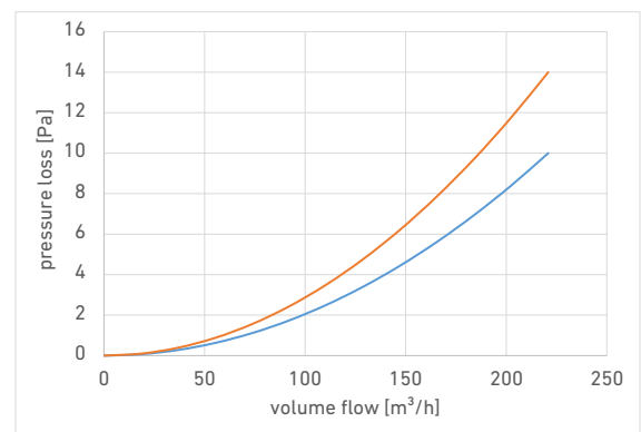
Pressure loss
