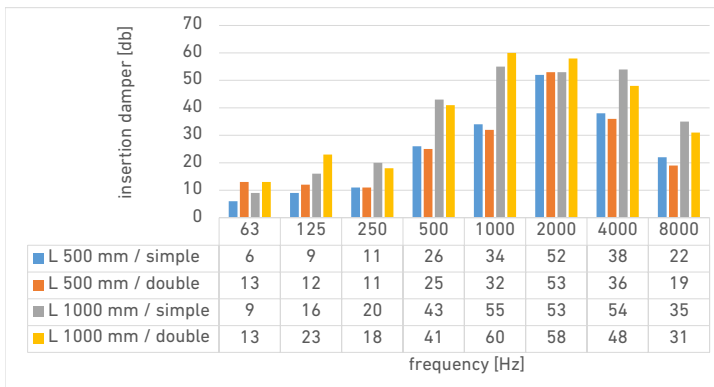
Insertion damper
