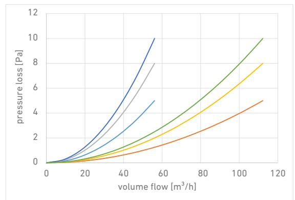
Pressure loss
