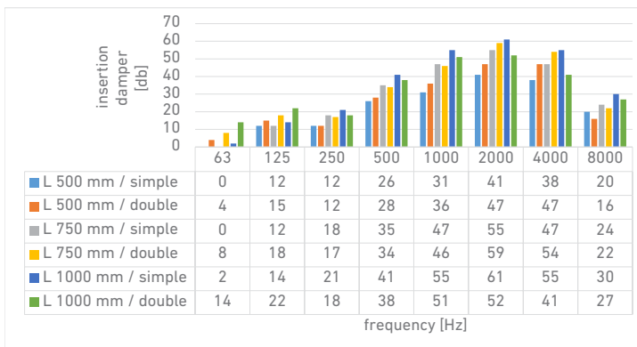
Insertion damper
