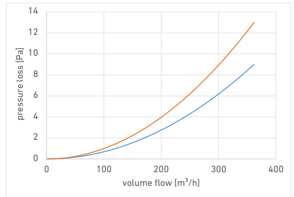
Pressure loss
