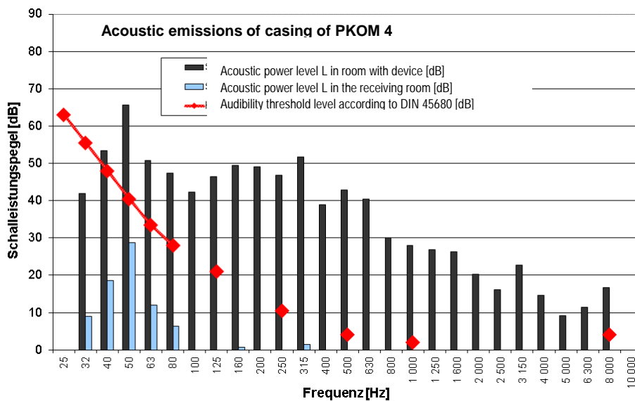
Figure 1: Noise emission of casing of unit PKOM 4 A
